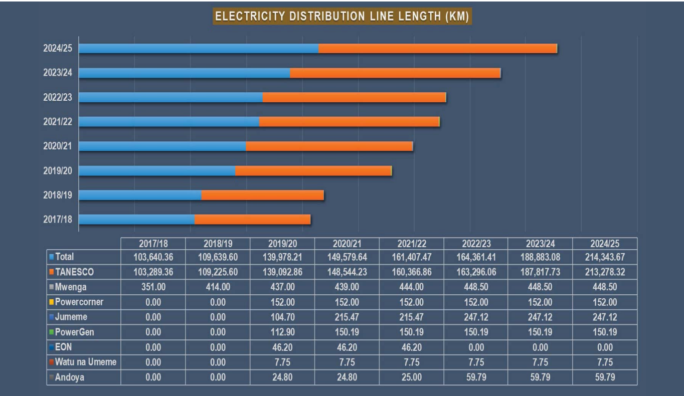
Figure 60: Electricity Distribution Line Length as of June 2025
