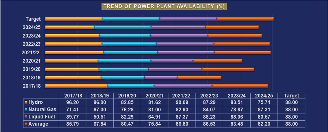
Figure 47: Power Plant Availability (%)
