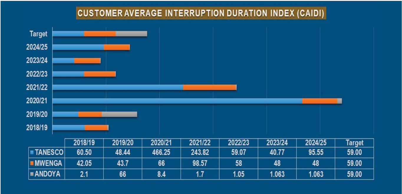
Figure 66: Customer Average Interruption Duration Index (CAIDI) in Minutes in FY2024/25
