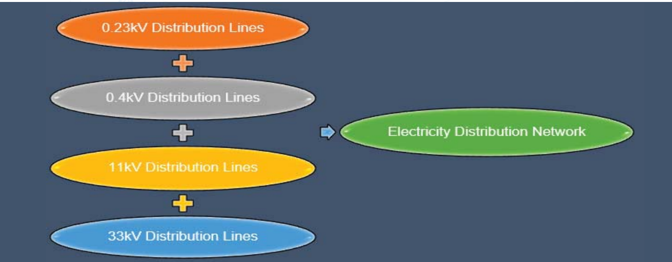
Figure 11: Electricity Distribution Network Voltage Levels as of June 2024
