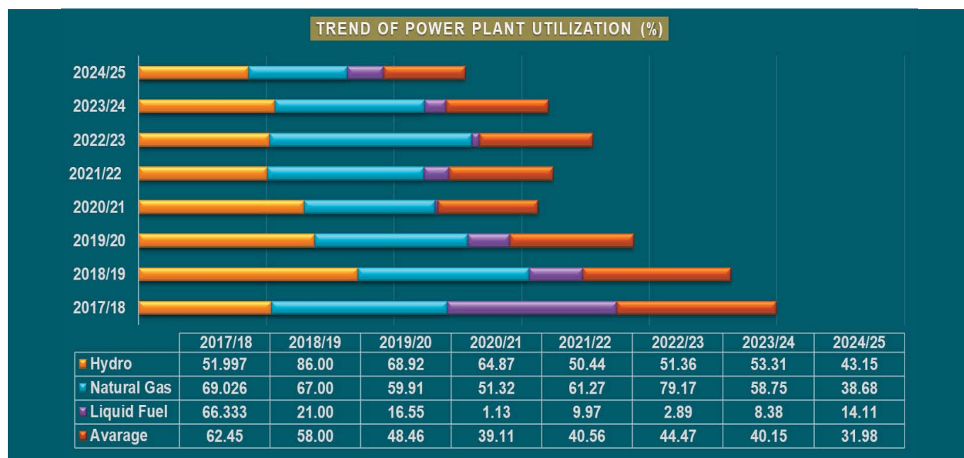
Figure 48: Power Plant Utilization (%)
