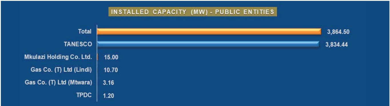
Figure 32: Contribution of Public Entities - Installed Capacity by June 2025
