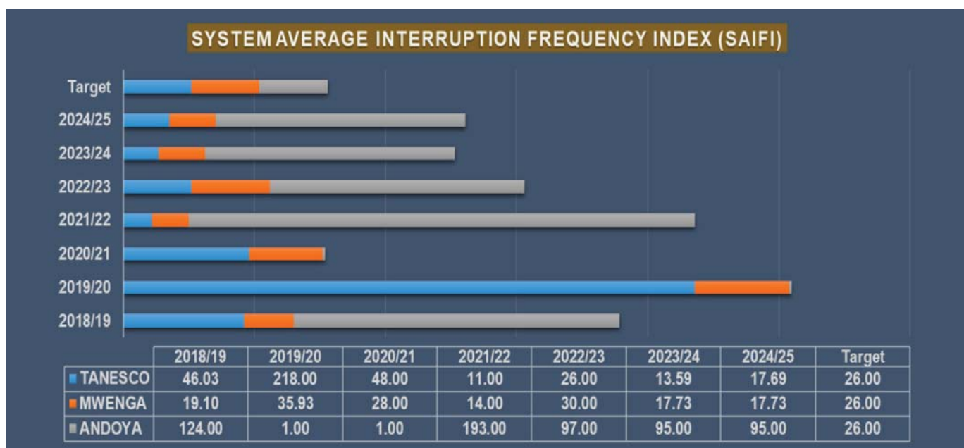
Figure 64: System Average Interruption Frequency Index (SAIFI) in FY2024/25
