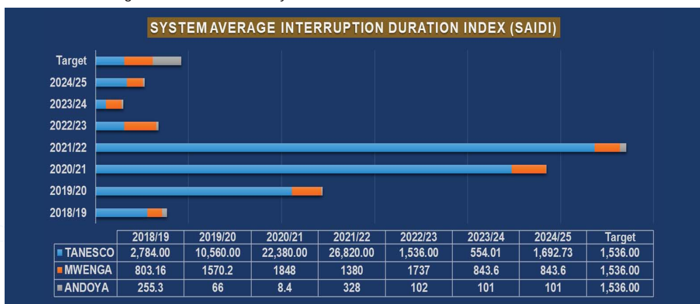
Figure 65: System Average Interruption Duration Index (SAIDI) in Minutes in FY2024/25
