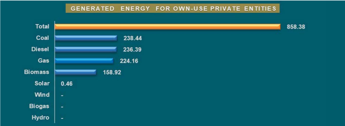
Figure 44: Energy Generation of Private Entities for Own-Use as Of June 2025
