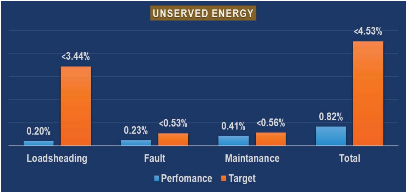
Figure 56: Unserved Energy in FY2024/25
