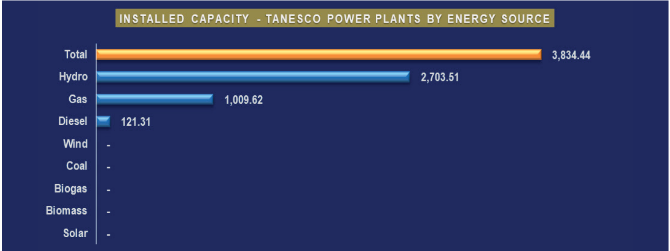
Figure 33: Installed Capacity of TANESCO Power Plants as Of June 2025
