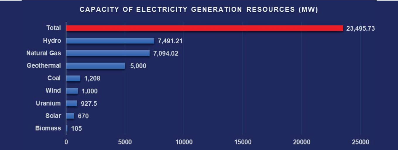
Figure 84: Capacity of Available Electricity Generation Resources (MW)
