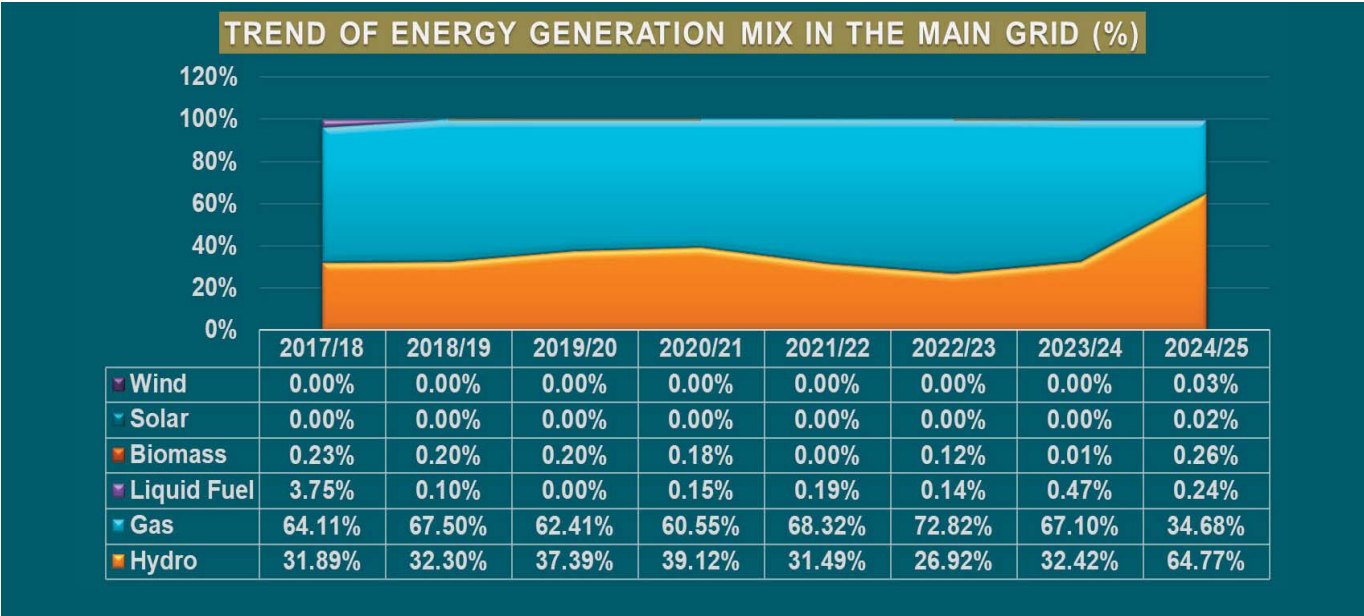
Figure 46: Energy Generation Mix (%) from FY 2017/18 – 2024/25
