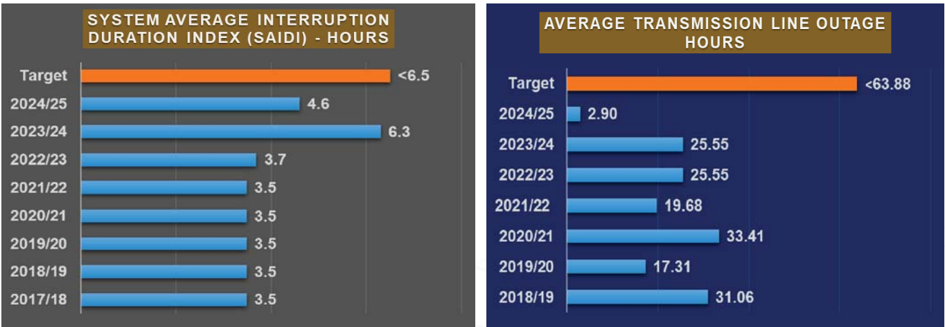
Figure 55: System Average Interruption Duration Index at Connection Point
